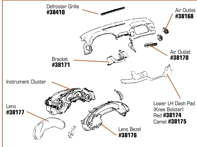
#38168 1997-2004 Far RH Air Duct Outlet
