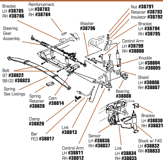
#38805 1997-2004 RH Front / LH Rear Knuckle
